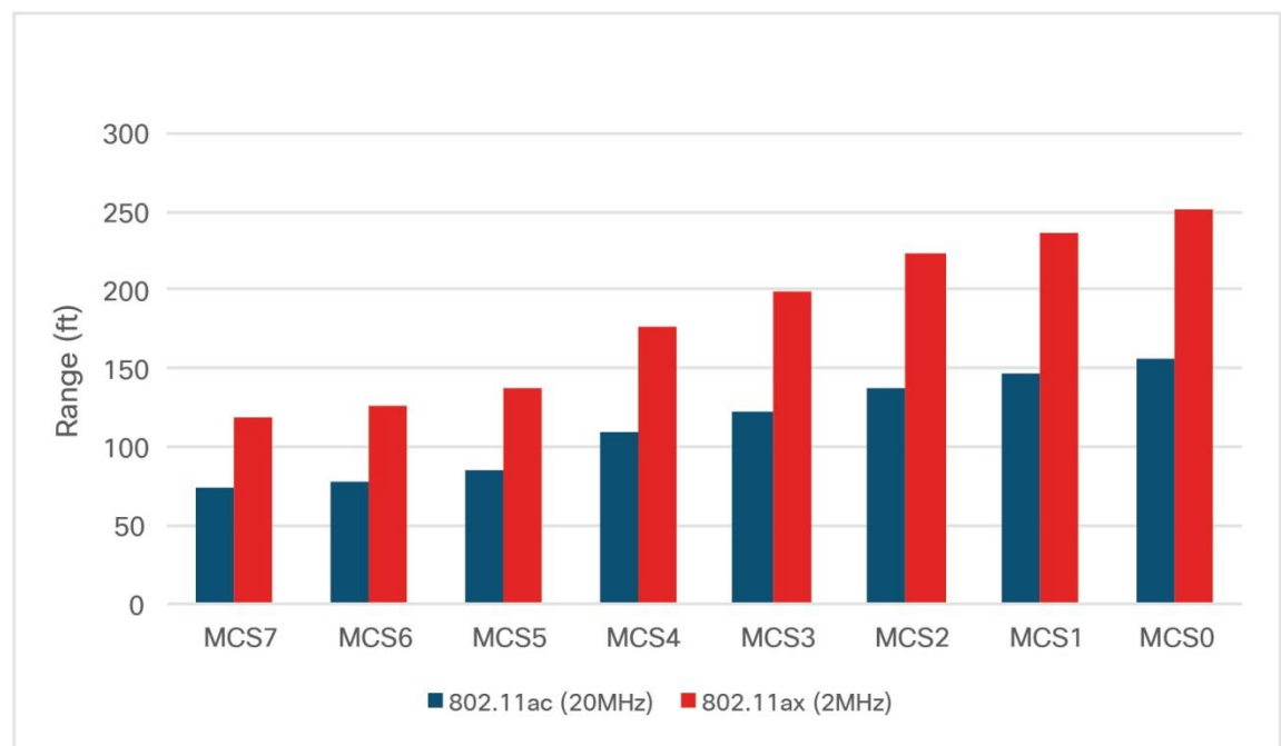
Figure 11. IEEE 802.11ax 2-MHz range boost (indoor 5-GHz NLOS)
