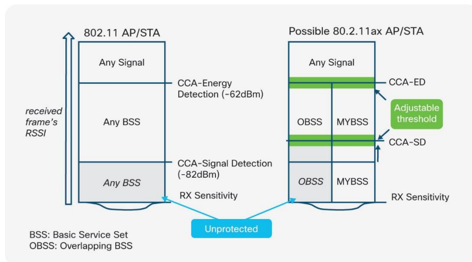
Figure 6. OBSS & BSS Color operation
