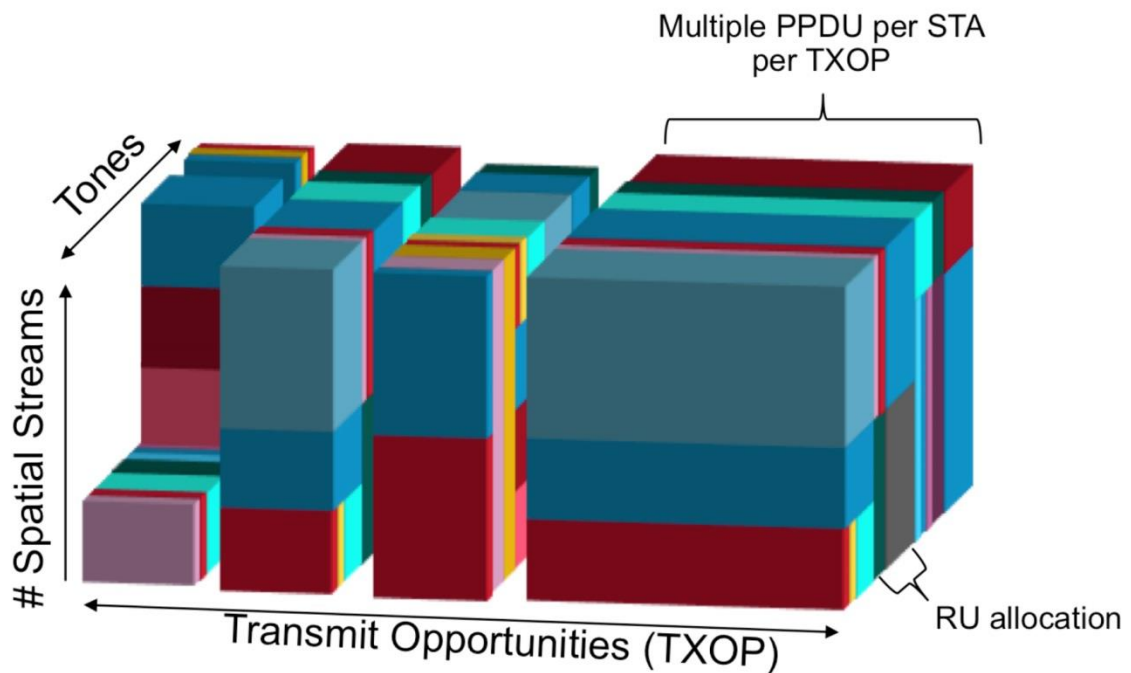
Figure 8. OFDMA resource dimensions
