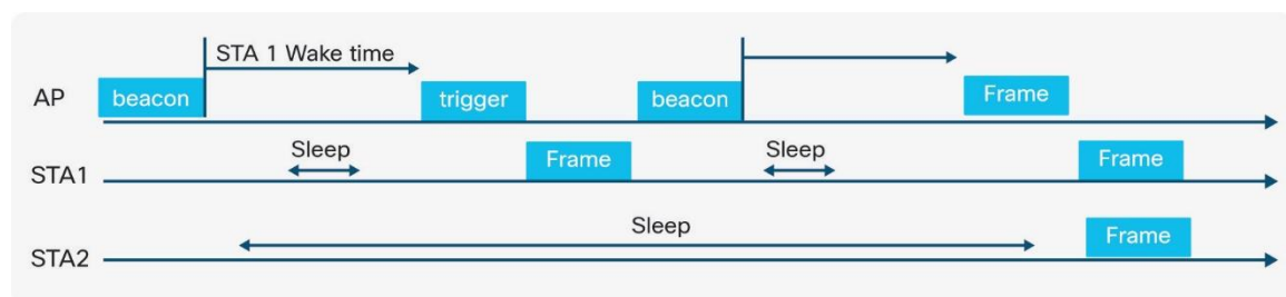
Figure 5. Target Wakeup Time (TWT) operation
