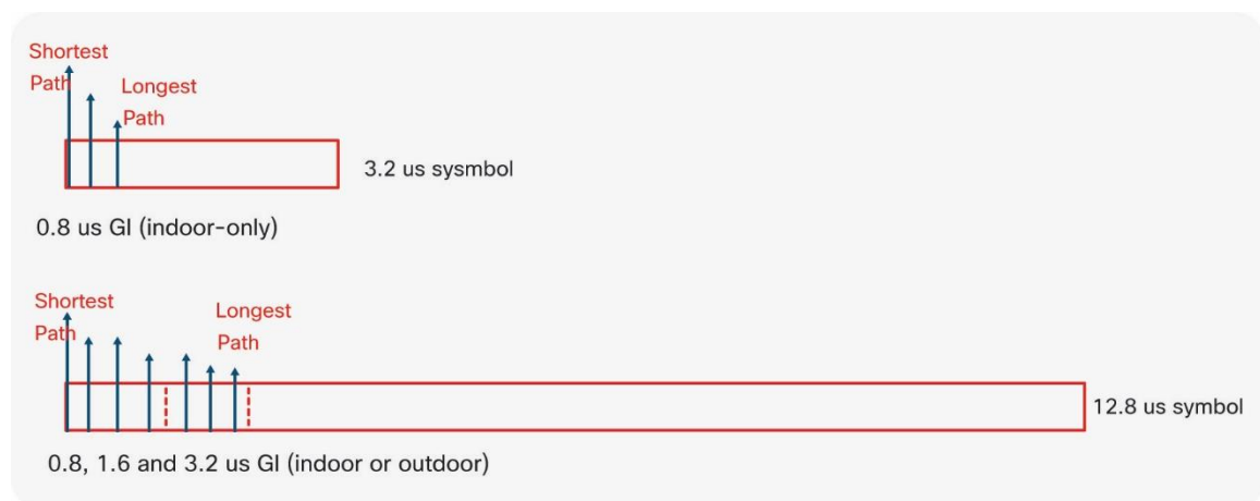
Figure 7. PHY timing options
