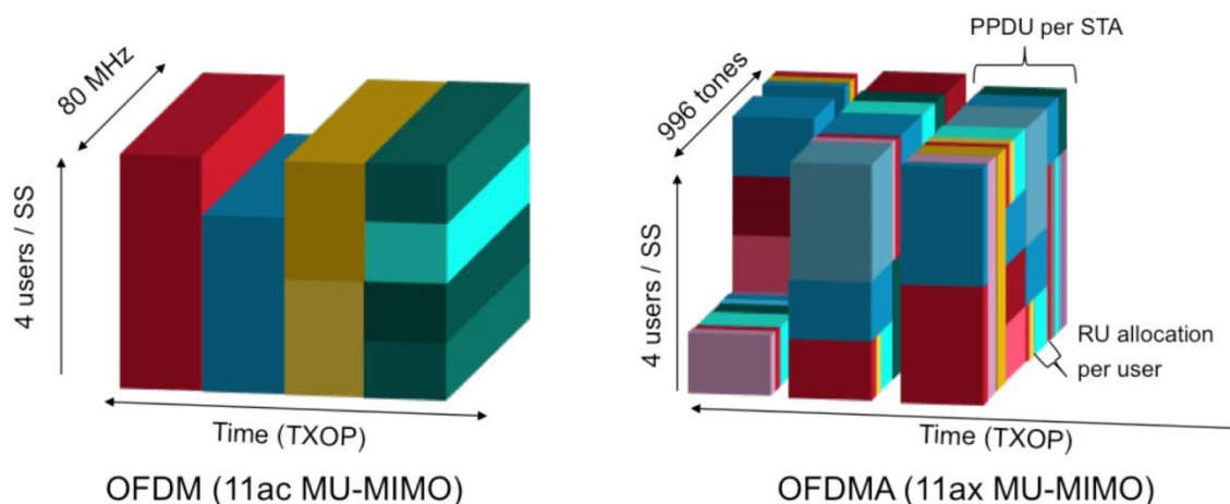
Figure 4. OFDM vs. OFDMA
