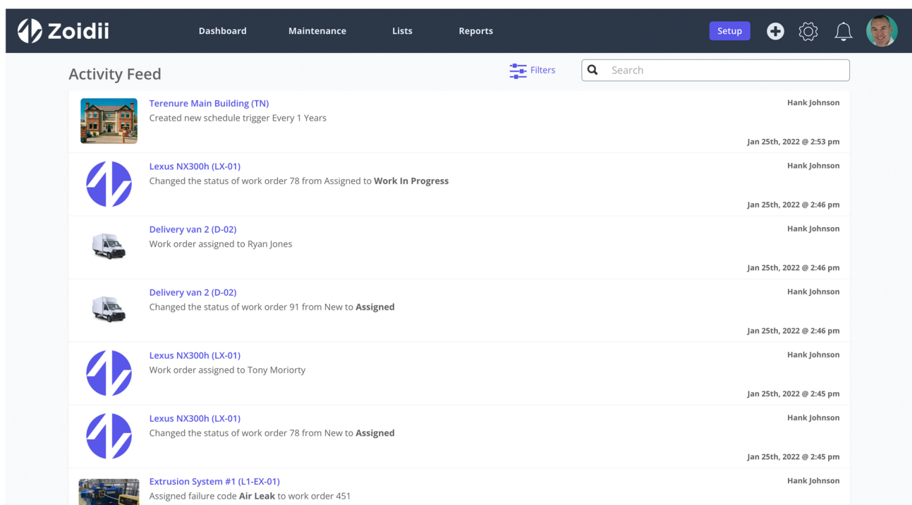
Fig. 5 - Activity View
