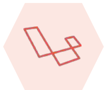
Laravel
