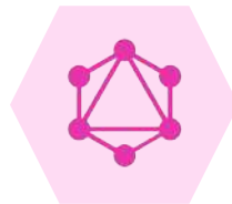
GraphQL
