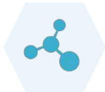
MolecularJS
